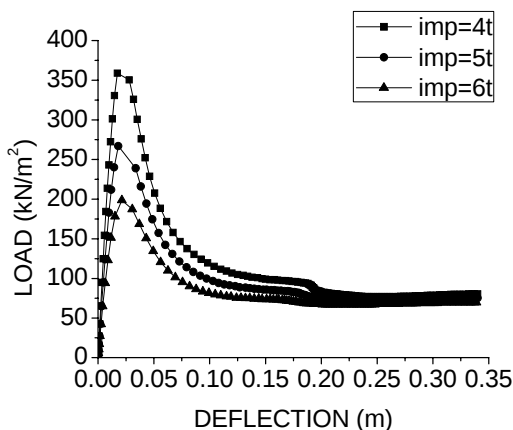
Fig. 6 Load-deflection curves of different magnitudes of initial geometrical imperfections for f/L = 1/4 .
