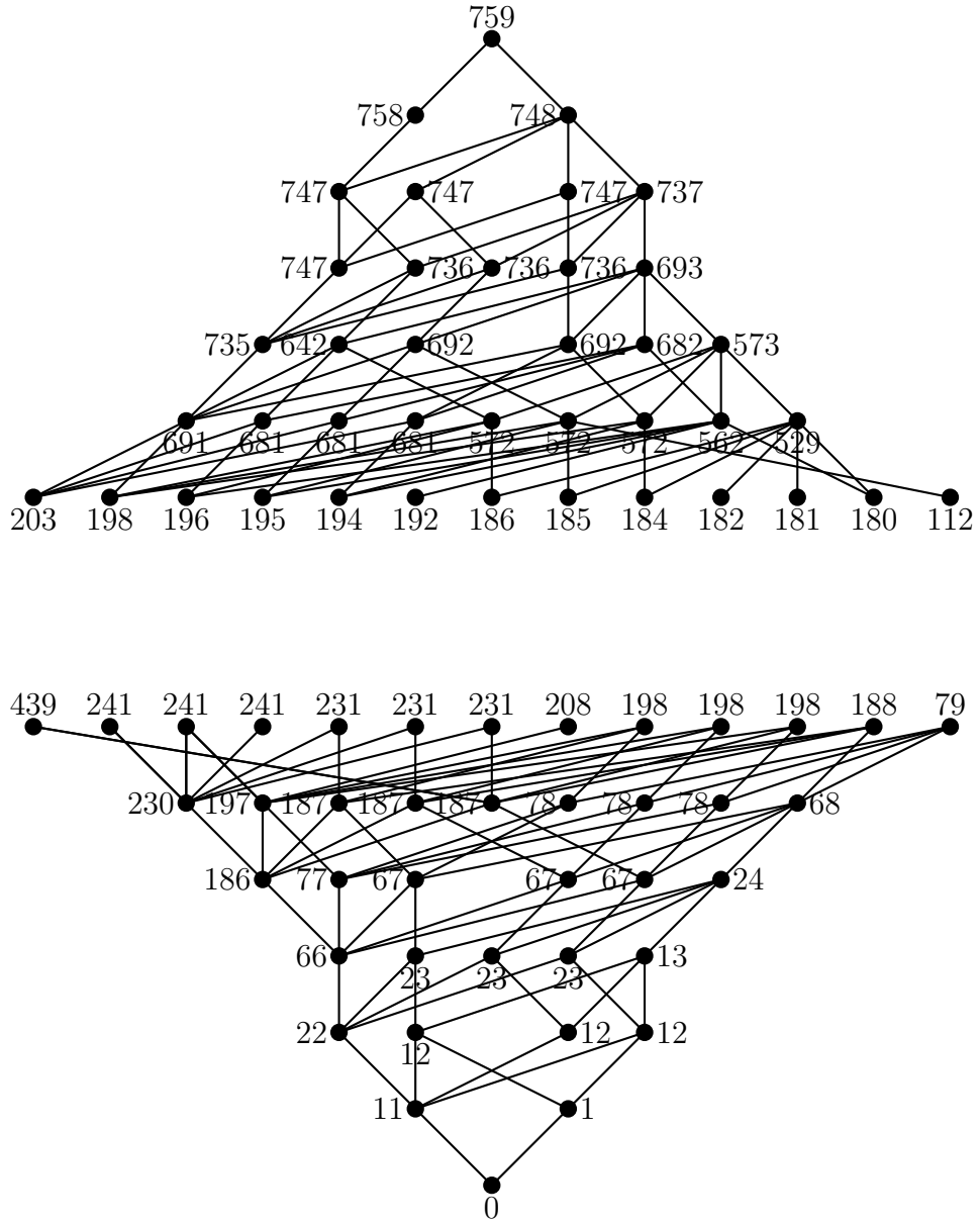
Figure 4.3: Partial Submodule lattice of degree 759
