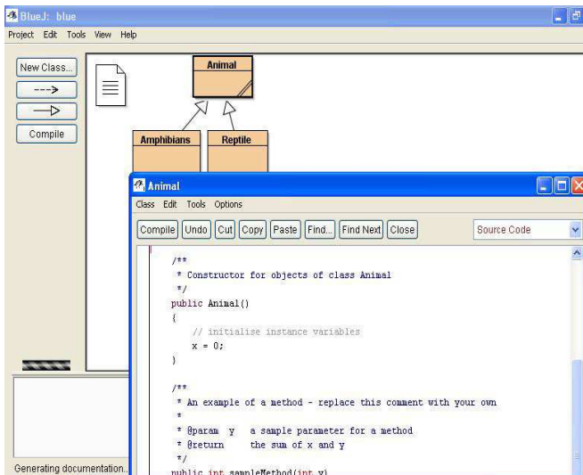
Fig. 3: BLUEJ Interface
