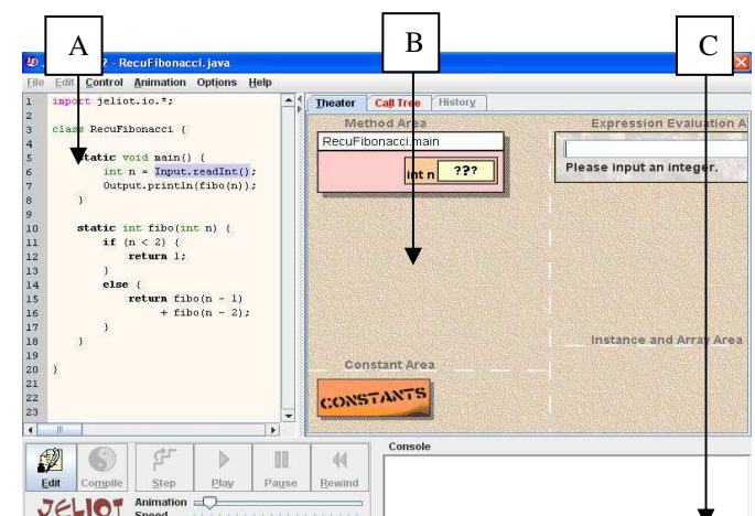
Fig. 2: JELIOT User Interface
