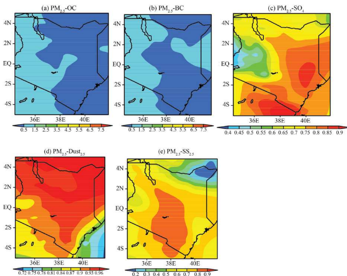
Figure 5. Spatial correlations of MERRA PM 2.5 and its components including (a) PM 2.5 -OC, (b) PM 2.5 -BC, (c) PM 2.5 -SO 4 , (d) PM 2.5 -Dust 2.5 , (e) PM 2.5 -SS 2.5 over Kenya during 1980 to 2020.
