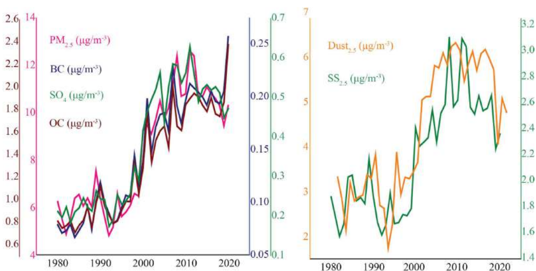
Figure 3. The annual mean trends in MERRA-2 \text{PM}_{2.5} and its five major components over Kenya from 1980 to 2020.
