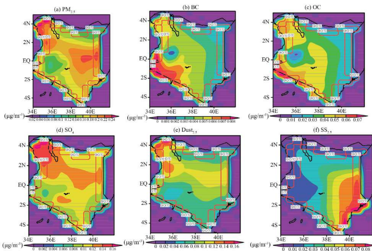
Figure 4. The annual trends of MERRA-2 PM_{2.5} and its individual components, including (a) the PM_{2.5} (b) Black Carbon PM_{2.5} (c) Organic Carbon PM_{2.5} (d) Sulphate PM_{2.5} (e) Dust PM_{2.5} (f) Sea Salt PM_{2.5} over Kenya during 1980-2020.
