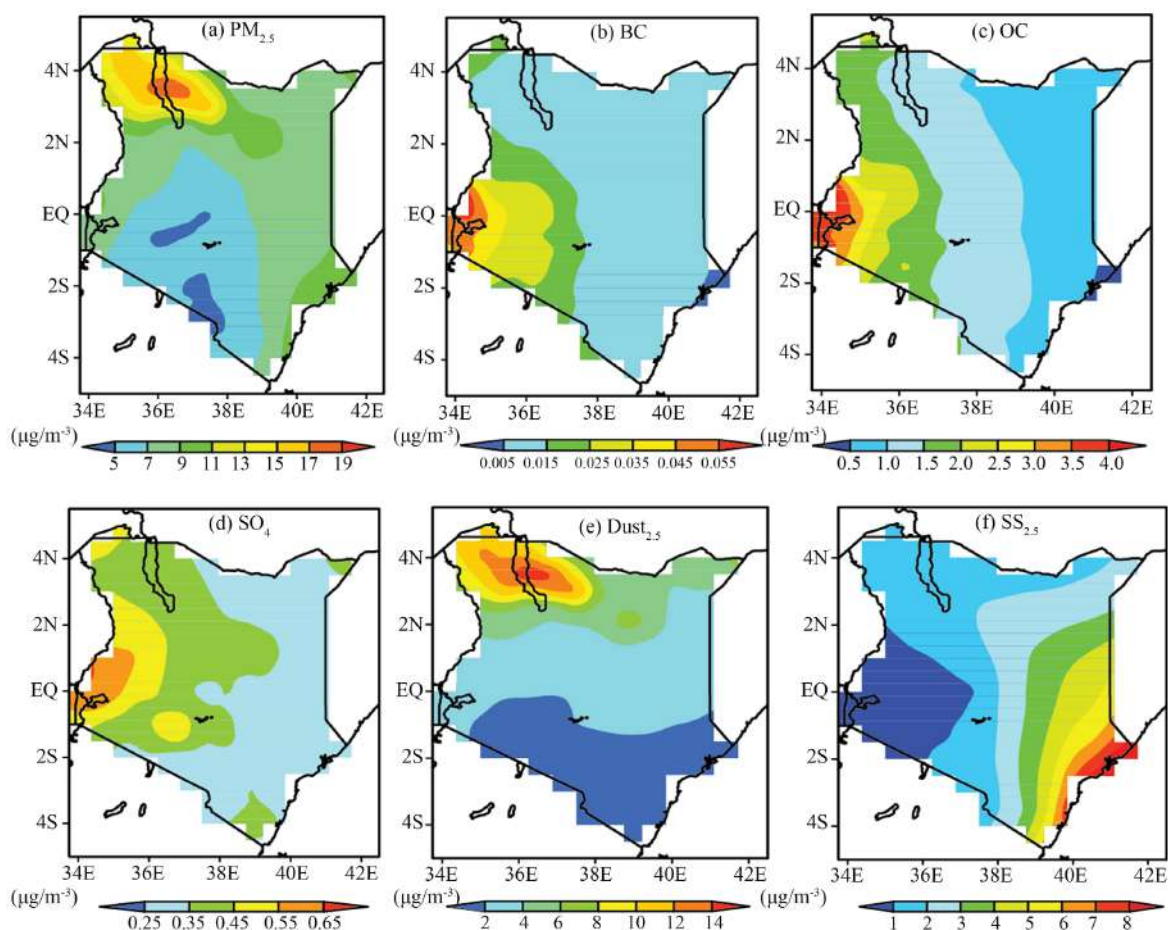
Figure 1. Spatial distribution of annual mean MERRA-2 \text{PM}_{2.5} and its components, including (b) Black Carbon (BC), (c) Organic Carbon (OC), (d) Sulphate ( \text{SO}_4 ), (e) Dust, (f) Sea Salt (SS) over Kenya during 1980-2020.
