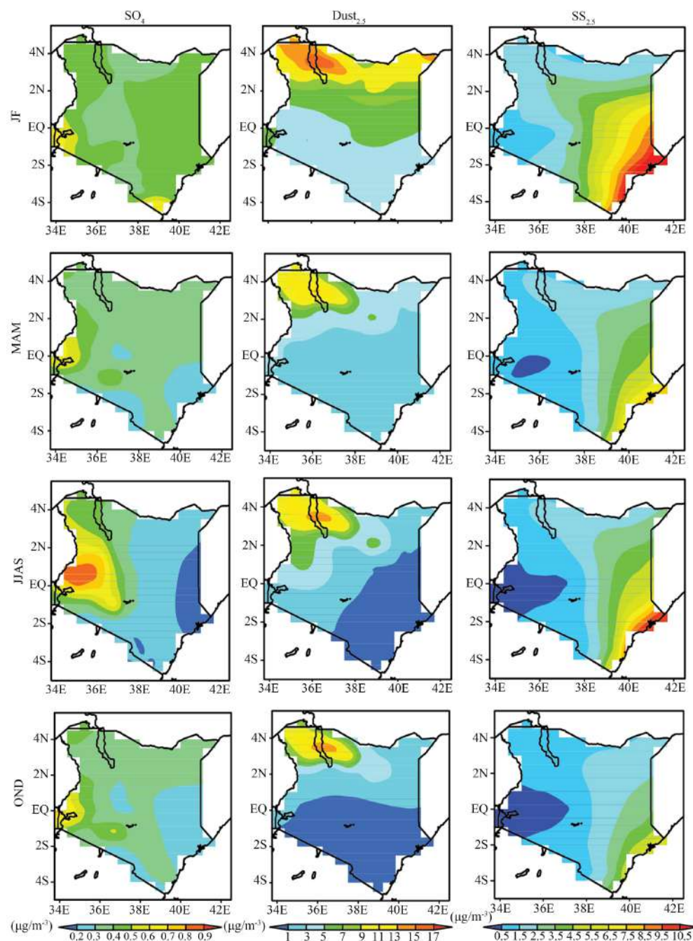
Figure 2. Seasonal variation of MERRA-2 PM_{2.5} and its components over Kenya during 1980-2020.
