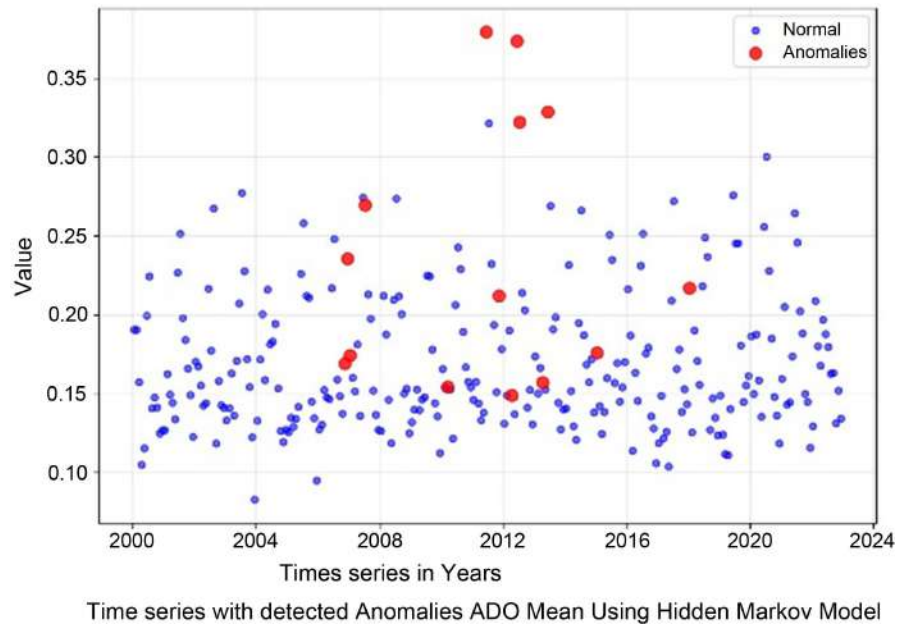
Figure 2. Time series with detected Anomalies AOD mean Using Hidden Markov Model (HMM) year 2000-2022.
