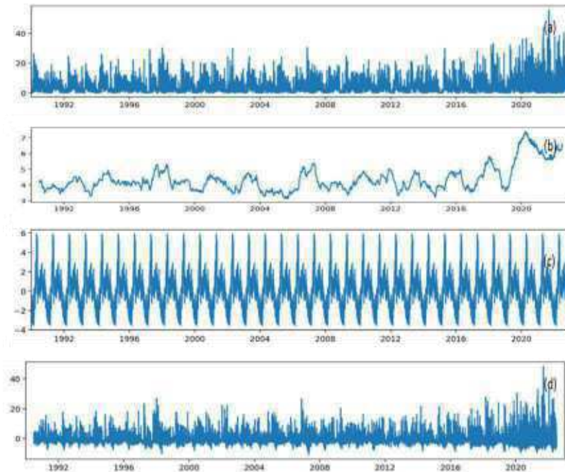
Figure 7. Seasonal Decomposition of Precipitation i.e. (a) Observed (b) Trend (c) Seasonality (d) Residual over Nandi County.
