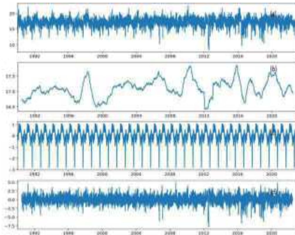
Figure 18. Seasonal Decomposition of Minimum Temperature i.e. (a) Observed (b) Trend (c) Seasonality (d) Residual over West Pokot County.
