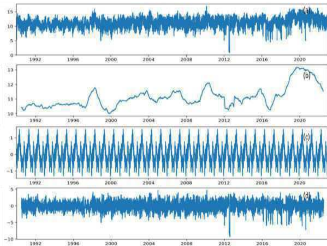
Figure 6. Seasonal Decomposition of Minimum Temperature i.e. (a) Observed (b) Trend (c) Seasonality (d) Residual over Uasin Gishu County.
