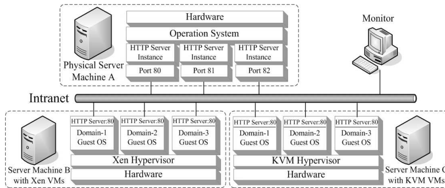
Experimental Setup: 3 configured systems, a non-virtualized server, a Xen-virtualized server, a KVM-virtualized server
