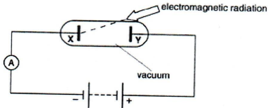
Figure 1: Showing an electrical circuit including a photocell
